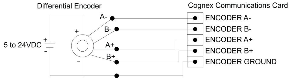
Figure A-7: Differential Encoder Configuration
