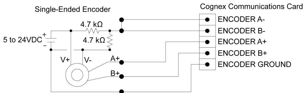
Figure A-8: Single-Ended Encoder Configuration
