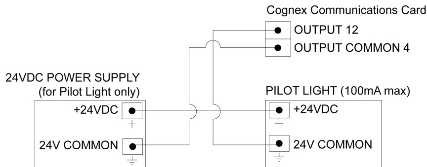
Figure A-5: Output to Pilot Light - Current Sinking
