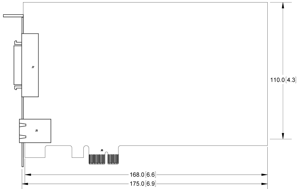
Figure 3-5: Communication Card Layout
