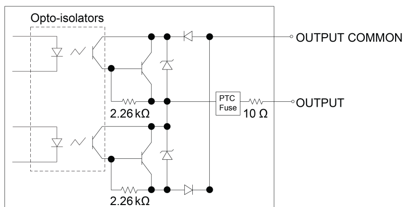
Figure 3-2: Output Schematic
