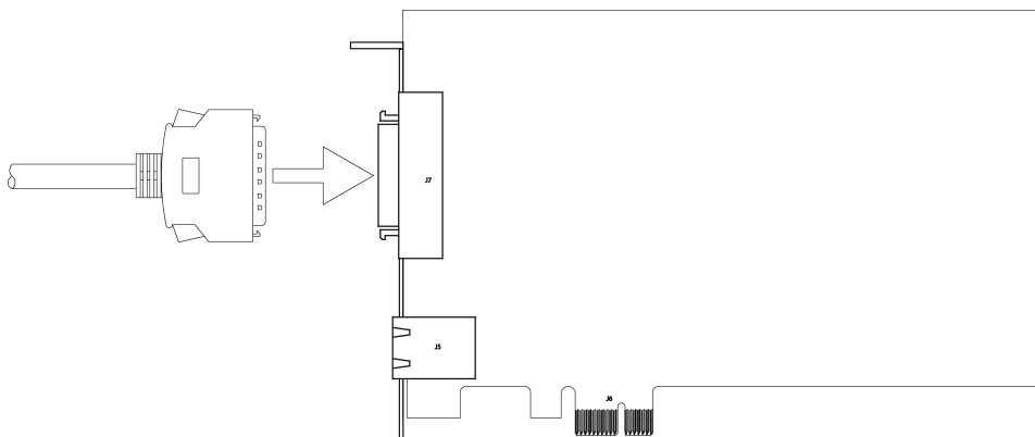
Figure 2-2: Connect the Breakout Cable
