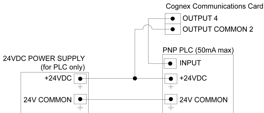
Figure A-4: Output to PLC - Current Sourcing
