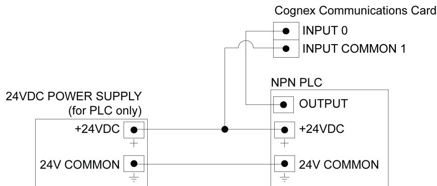
Figure A-1: Input from PLC - Current Sinking
