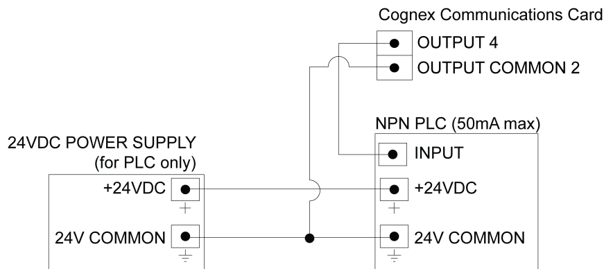
Figure A-3: Output to PLC - Current Sinking
