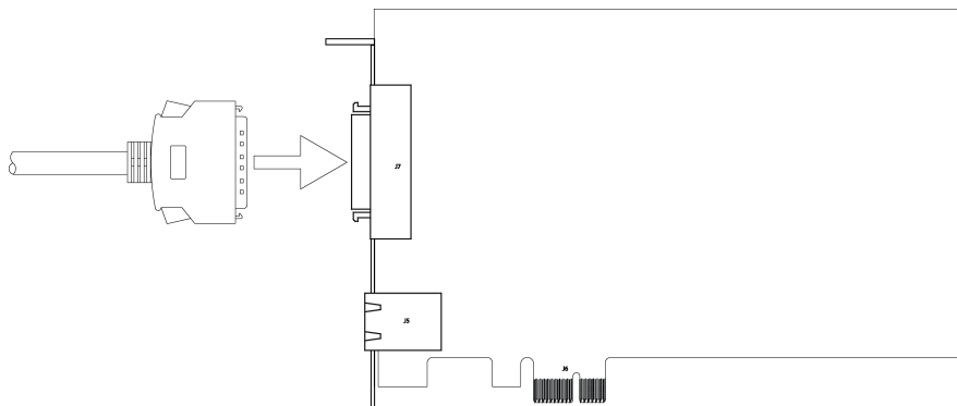
Figure 2-3: Connect the I/O Terminal Block Cable
