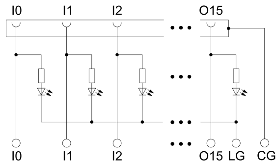
Figure 3-4: LED Schematic
