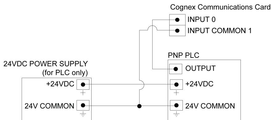
Figure A-2: Input from PLC - Current Sourcing
