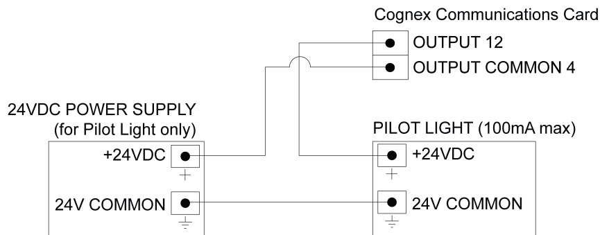
Figure A-6: Output to Pilot Light - Current Sourcing
