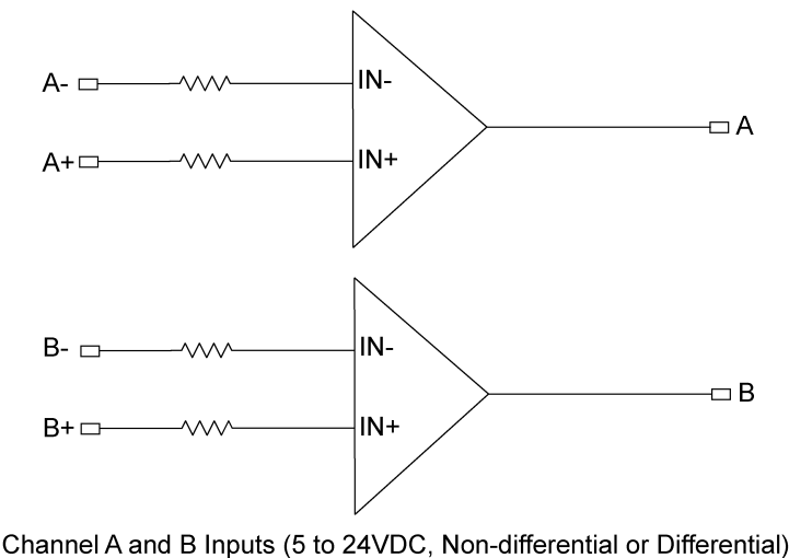
Channel A and B Inputs (5 to 24VDC, Non-differential or Differential) Figure 3-3: Channel A and Channel B Inputs
