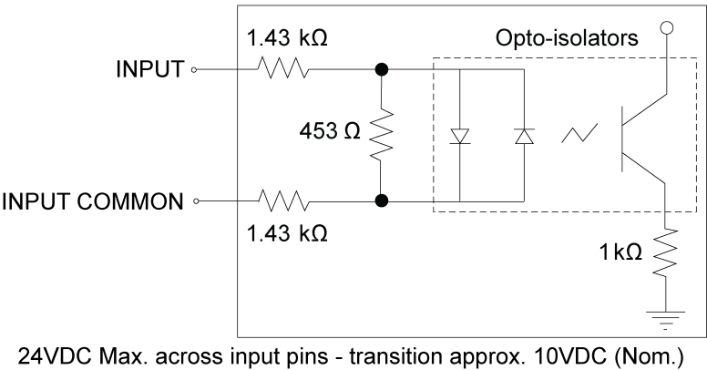
Figure 3-1: Input Schematic
